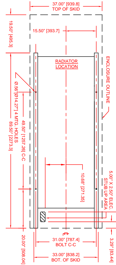
ENCLOSURE / GENERATOR FLOOR MTG. PLAN ALLOW 38" AT SIDES OF ENCLOSURE FOR DOOR OPENINGS
