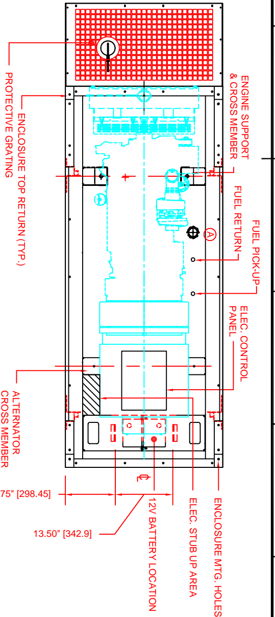
PLAN VIEW SHOWN WITHOUT ROOF
