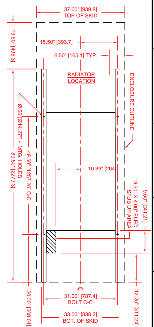
ENCLOSURE / GENERATOR FLOOR MTG. PLAN ALLOW 38" AT SIDES OF ENCLOSURE FOR DOOR OPENINGS
