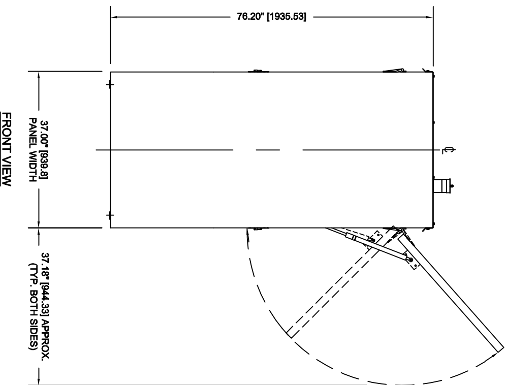
ENCLOSURE / GENERATOR FLOOR MTG. PLAN ALLOW 38" AT SIDES OF ENCLOSURE FOR DOOR OPENINGS
