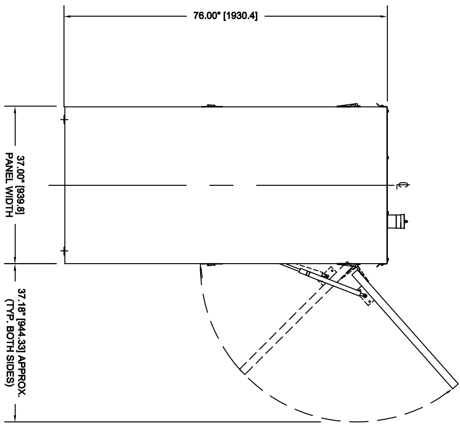
BOTTOM OF FUEL TANK FLOOR MOUNTING PLAN LOOKING DOWN, ALLOW 38" AT SIDE FOR DOOR OPENING.
