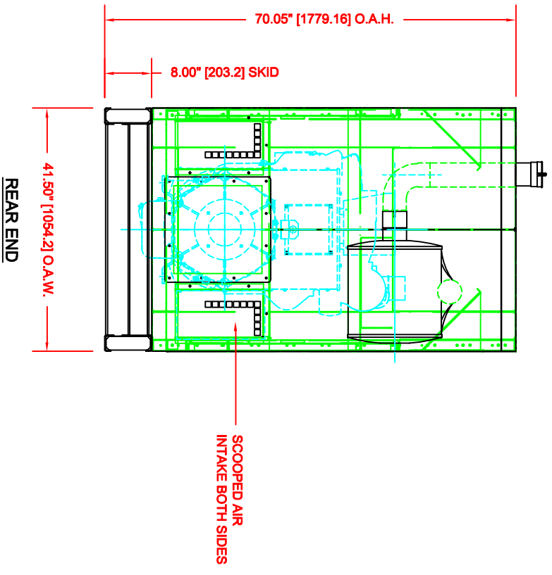
ENCLOSURE / GENERATOR FLOOR MTG. PLAN / TOP VIEW ALLOW 37" AT SIDES OF ENCLOSURE FOR DOOR OPENINGS
