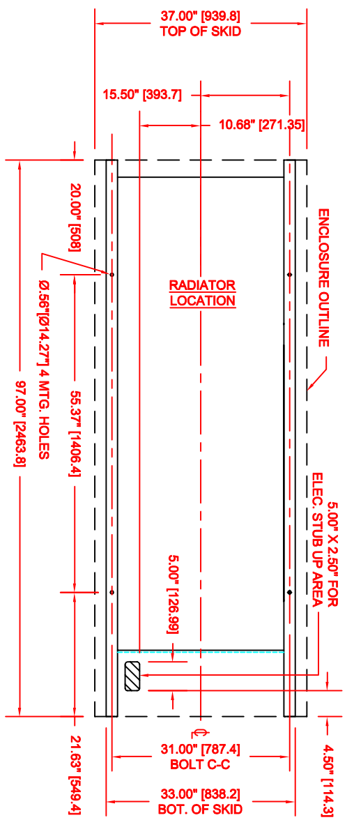
ENCLOSURE / GENERATOR FLOOR MTG. PLAN ALLOW 38" AT SIDES OF ENCLOSURE FOR DOOR OPENINGS
